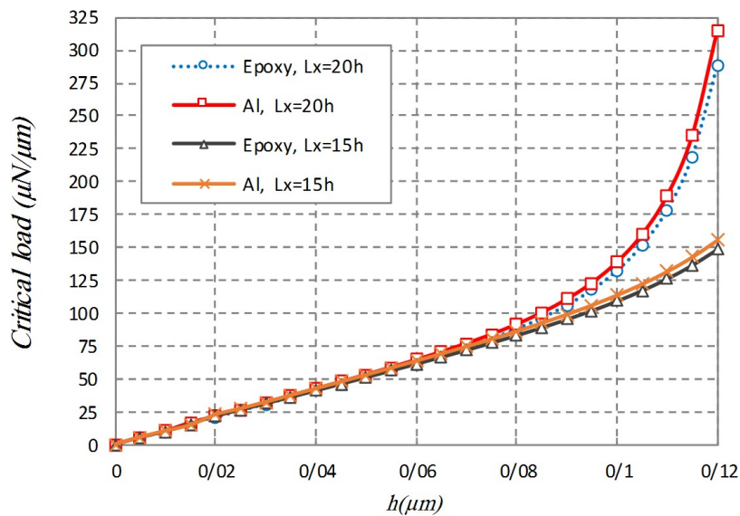
Fig. 5. Variation of the panel thickness versus various core materials ( \beta=1, \eta=1, L_x=15h, k_1=k_2=1, l=0.5h, m=n=1, \text{CFCF} )
