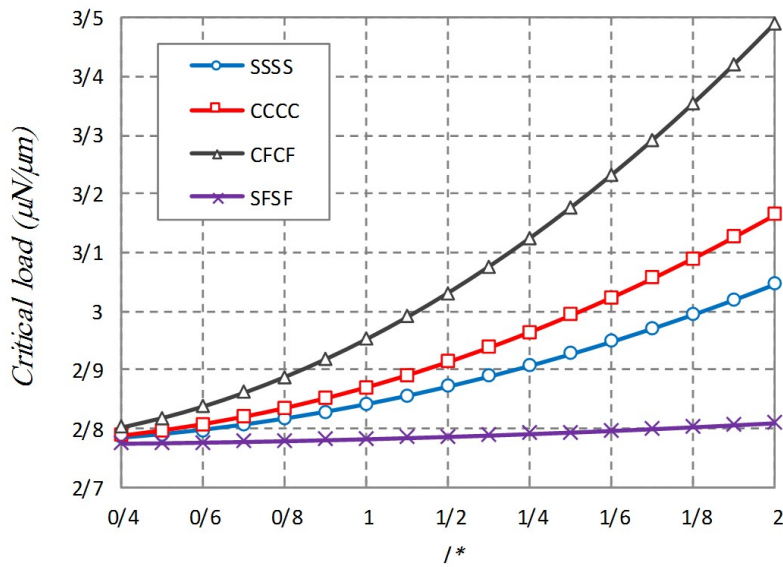
Fig. 4b. Length scale parameter versus boundary conditions ( \beta=1, T=0.1, L_x=20h, \eta=0, k_1=k_2=1, l^*=l/h, m=n=1, \text{Epoxy} )
