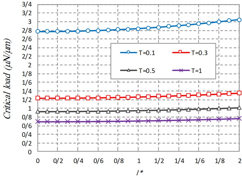
Fig. 4a. The length scale parameter versus the thickness ( \beta=1, T=t_1/t_2, L_x=20h, \eta=0, k_1=k_2=1, l^*=l/h, m=n=1, \text{SSSS, Epoxy} )
