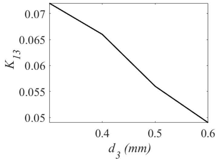
Figure 12. Variation of coupling coefficient K_{13} .
