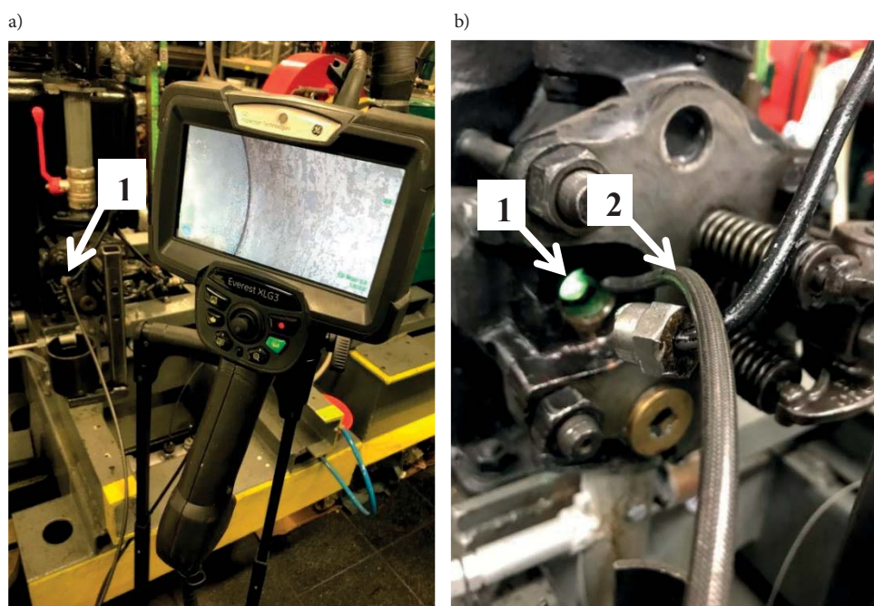
Fig. 3. View of the XLG3 manual endoscope panel with a visible image of the cylinder space of the Farymann Diesel research engine type D10 (a) way of inserting the inspection probe of the video endoscope into the research engine working space (b) 1 - inspection hole after removing the fuel injector, 2 - inspection probe
