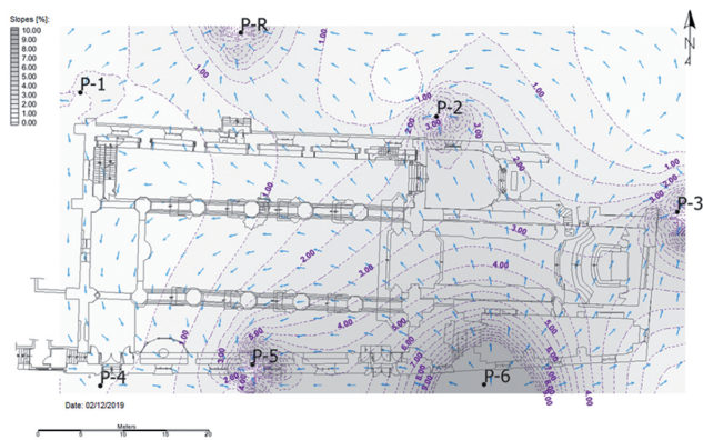
Fig. 12. Map of local groundwater table declines with seepage directions for 2/12/2019, against the background of the Basilica basement level plan
