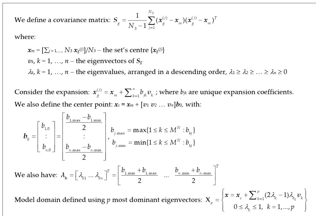
Figure 3. Procedure for surrogate domain identification with dimensionality reduction using spectral analysis of the observable set [85] (for details see [43]). Notation: S_g —covariance matrix, N_3 —the number of the pre-optimized designs with the lowest constraint violation; \{\mathbf{x}_g^{(j)}\} —the observable set; \mathbf{x}_m —the center of the observable set; \mathbf{x}_c —the center point; \mathbf{v}_k —the eigenvectors of S_g ; \lambda_k —the eigenvalues of S_g ; b_{jk} —expansion coefficients.
