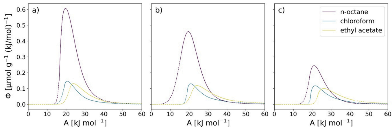
Fig. 8. Adsorption potential distribution for aerogels samples prepared at -116 \text{ }^\circ\text{C} hydrogel freezing temperature and different concentrations: a) 2 \text{ mg mL}^{-1} , b) 6 \text{ mg mL}^{-1} , c) 10 \text{ mg mL}^{-1} . Solid lines represent the part of distribution covered by experimental data. Dashed line is an extrapolation using split-Pearson VII distribution.
