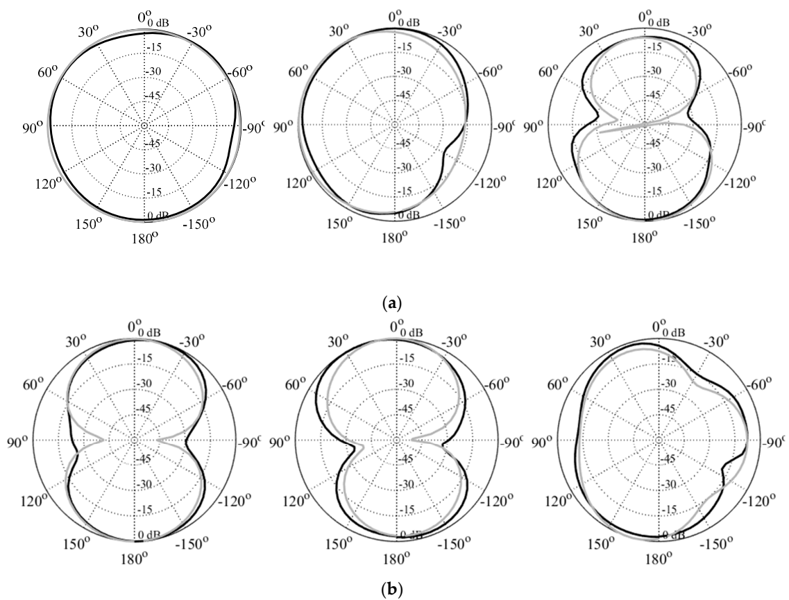
Figure 46. Experimental validation of the triple-band antenna of Figure 27: (a) simulated (gray) and measured (black) yz -plane patterns; (b) simulated (gray) and measured (black) yz -plane patterns. Patterns shown correspond to 4.0 GHz (left), 6.0 GHz (middle), and 8.0 GHz (right).
