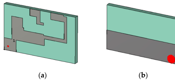
Figure 27. Illustration case IV: 25 × 15 mm ultra-wideband antenna: (a) front view; (b) back view.
