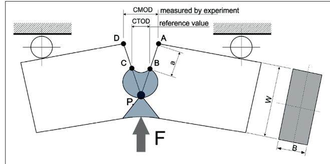
Fig. 2. Principle of the CTOD test
