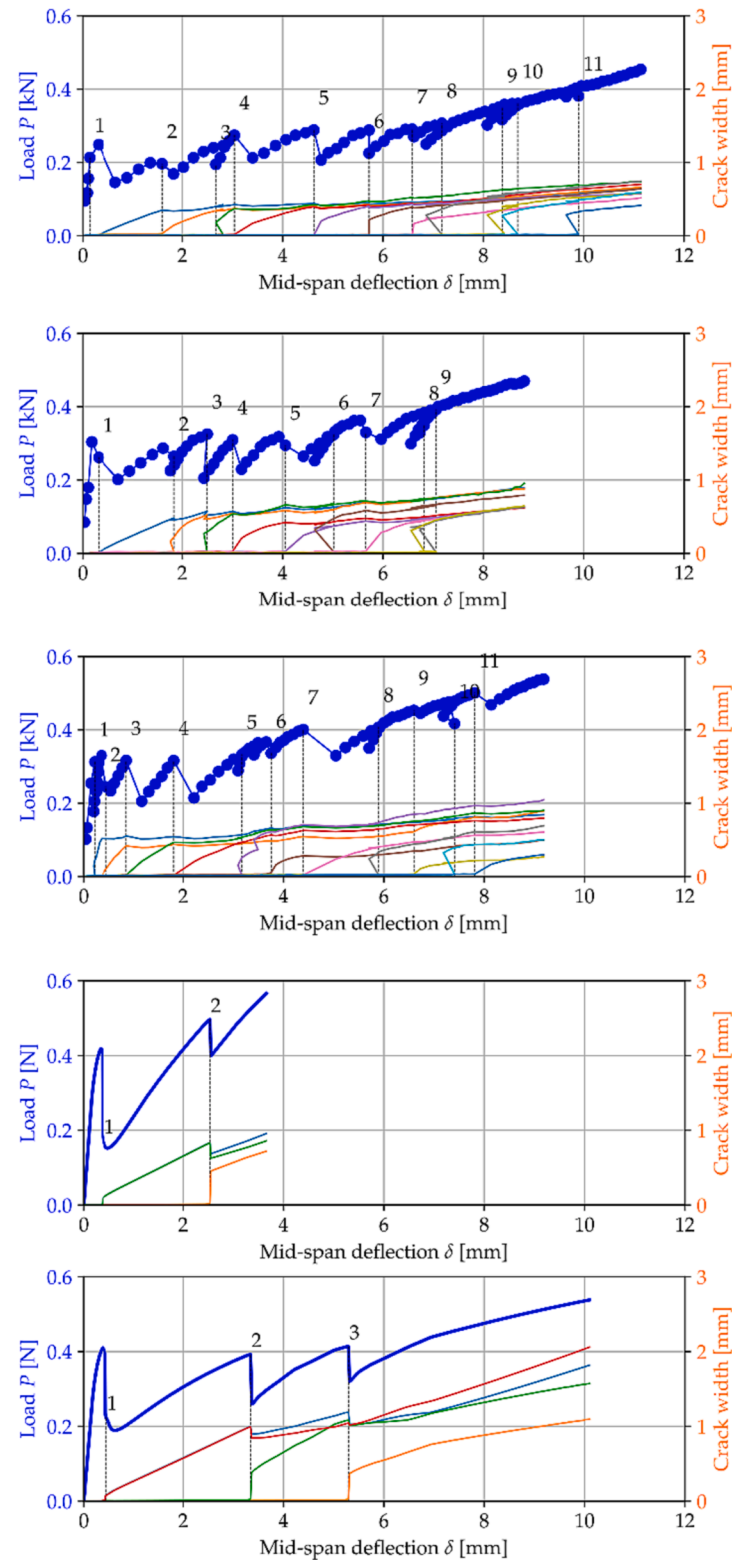
Fig. 14. Experimental (Oa, Ob, Oc) and numerical (Input I and Input II) results of one-way flexure tests. Left: Contour plots of the main principal strain at maximum load (P as defined in Fig. 8). The placement of the textile mesh is indicated. Cracks are numbered in order of appearance. Right: Load and crack widths versus mid-span deflection relative to the deflection at the load positions, see Fig. 3.
