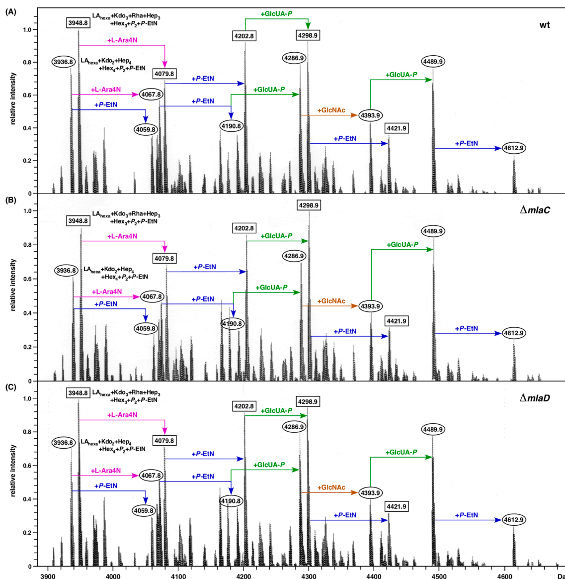
Figure 7. In the absence of either the mIaC or mIaD gene, LPS structure is similar to that of parental wild type. Charge-deconvoluted mass spectra in the negative ion mode of LPS from the wild type (A) and its \Delta mIaC (B) and \Delta mIaD (C) derivatives. Cultures were grown in phosphate-limiting medium at 30 °C. Mass numbers refer to monoisotopic peaks. Mass peaks with rectangular boxes correspond to the glycoform containing the third Kdo. Mass peaks marked with an oval box correspond to predicted LPS containing two Kdo residues.
