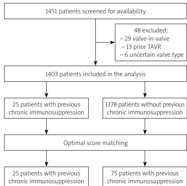
Figure 1. Study flowchart
