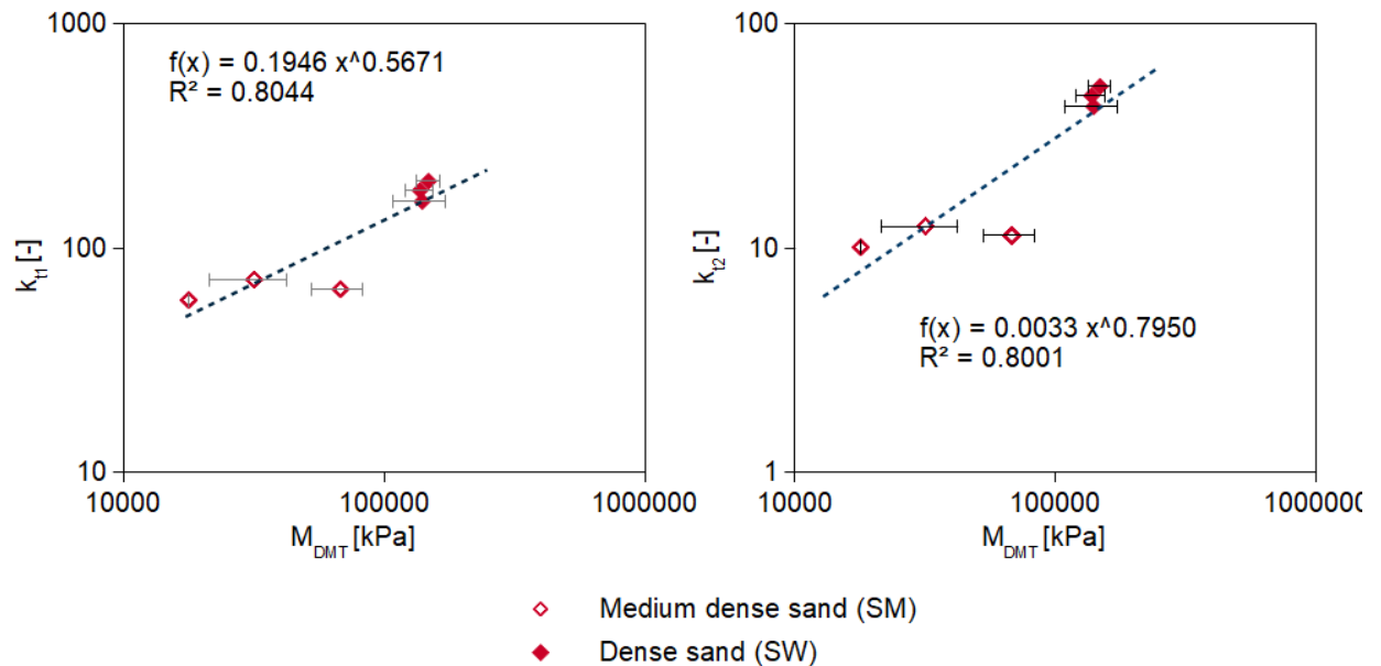
Figure 7.29. Relationship between coefficients k_{t1} and k_{t2} and dilatometer modulus M_{DMT} for non-cohesive soils on rough concrete.
