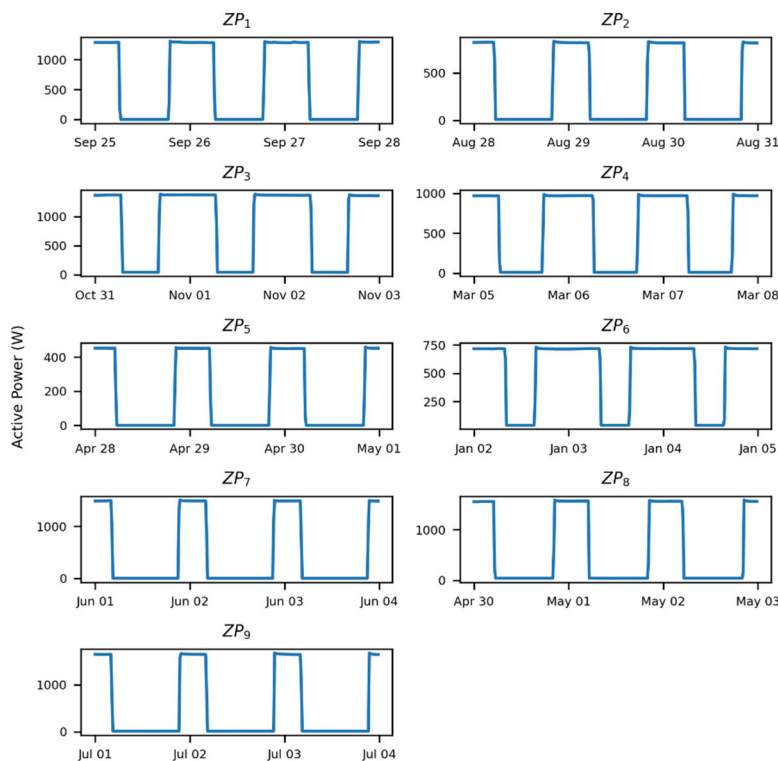
FIGURE 6. Example visualizations of power measurement data for ZP 1 , ZP 2 , ...ZP 9 .
