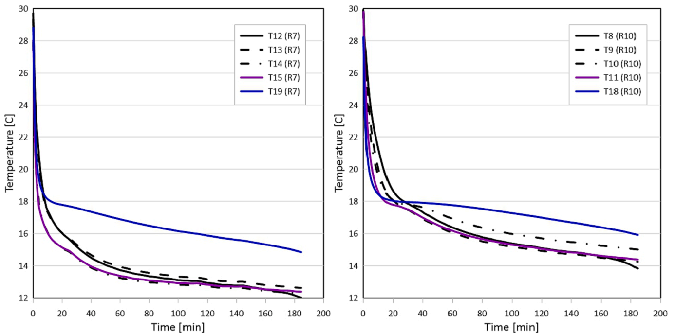
Fig. 7. Temperature profile for solidification of RT18HC for constant wall temperature ( T_w = 10.5C ): at left for R = 7 mm; at right for R = 10 mm.
