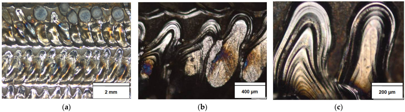
Figure 9. Untreated AISI 316L surface subjected to laser texturing of 2500 W laser beam power with pulse focus of 0.5 mm and frequency of 3 Hz: (a) 10× magnification by ZEISS; (b) 50× magnification by Olympus; and (c) 100× magnification by Olympus.
