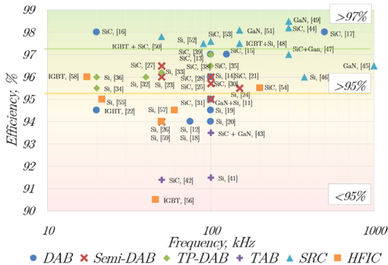
Fig.5. Comparison of converters switching frequencies.
