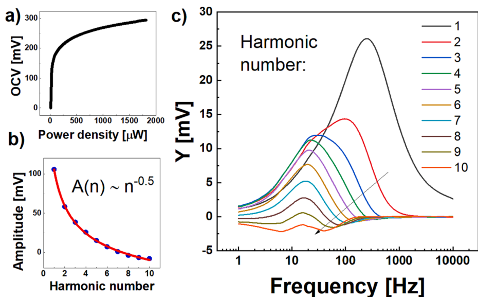
Fig. 6. A) Photovoltage dependence on the illumination intensity, b) decay profile of the IMVS amplitude at the low-frequency limit, c) imaginary part of higher harmonics of IMVS spectra from 1 to 10, arrows indicate the increasing number of harmonics.
