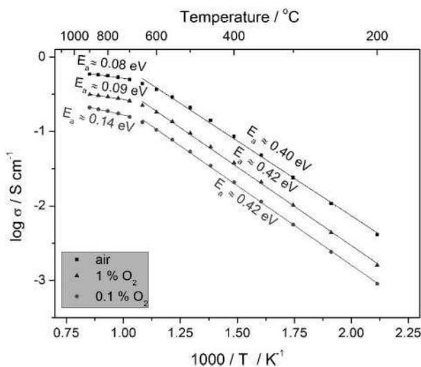
Fig. 2 – Electrical conductivity plots of sintered STF35 pellet in 21%, 1% and 0.1% O_2 .
