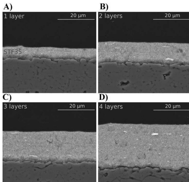
Figure 7. The SEM images of the polished cross section of the sintered at 800\ ^{\circ}C STF35 porous layers with different thickness (A-D) on the Al_2O_3 substrate.
