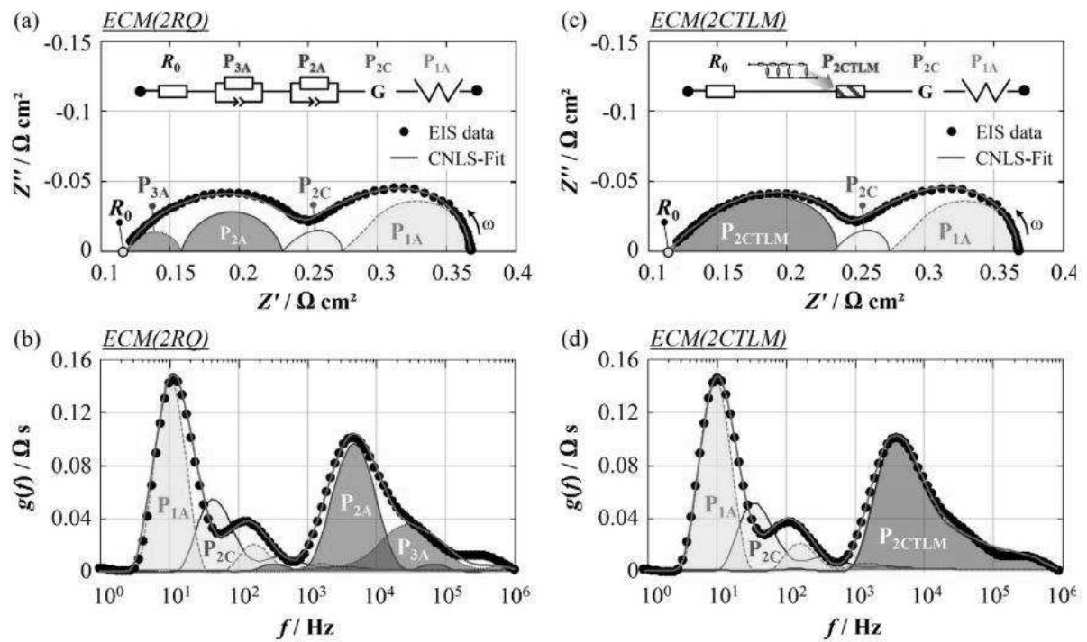
Figure 9. Measured and simulated impedance spectra and DRTs of an anode-supported SOFC based on different equivalent circuit models. Figures (a) and (b) are simulated with the established ECM with two RQ-elements – ECM(2RQ). In (c) and (d), the two RQ-elements are substituted by a physical parametrised TLM model – ECM(2CTLM). The cathode processes are blue and the anode processes are red. The measurement was recorded under OCV-conditions at 720 °C, with 20% humidified hydrogen as fuel and ambient air as oxidant [67].
