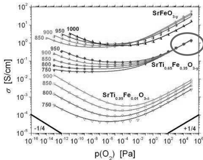
Figure 7. Total conductivity isotherms at different temperatures (750–1000 °C) as a function of oxygen partial pressure ( p(\text{O}_2) ) for STF compositions with 1 mol % (STF01), 35 mol % (STF35), and 100 mol % Fe ( \text{SrFeO}_{3-y} ). Experimental data points are represented by symbols, fitted curves by solid lines [46].
