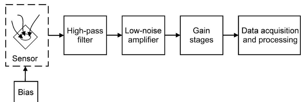
Figure 4. Schematic of a measurement setup for low-frequency noise measurements (LFNM).
