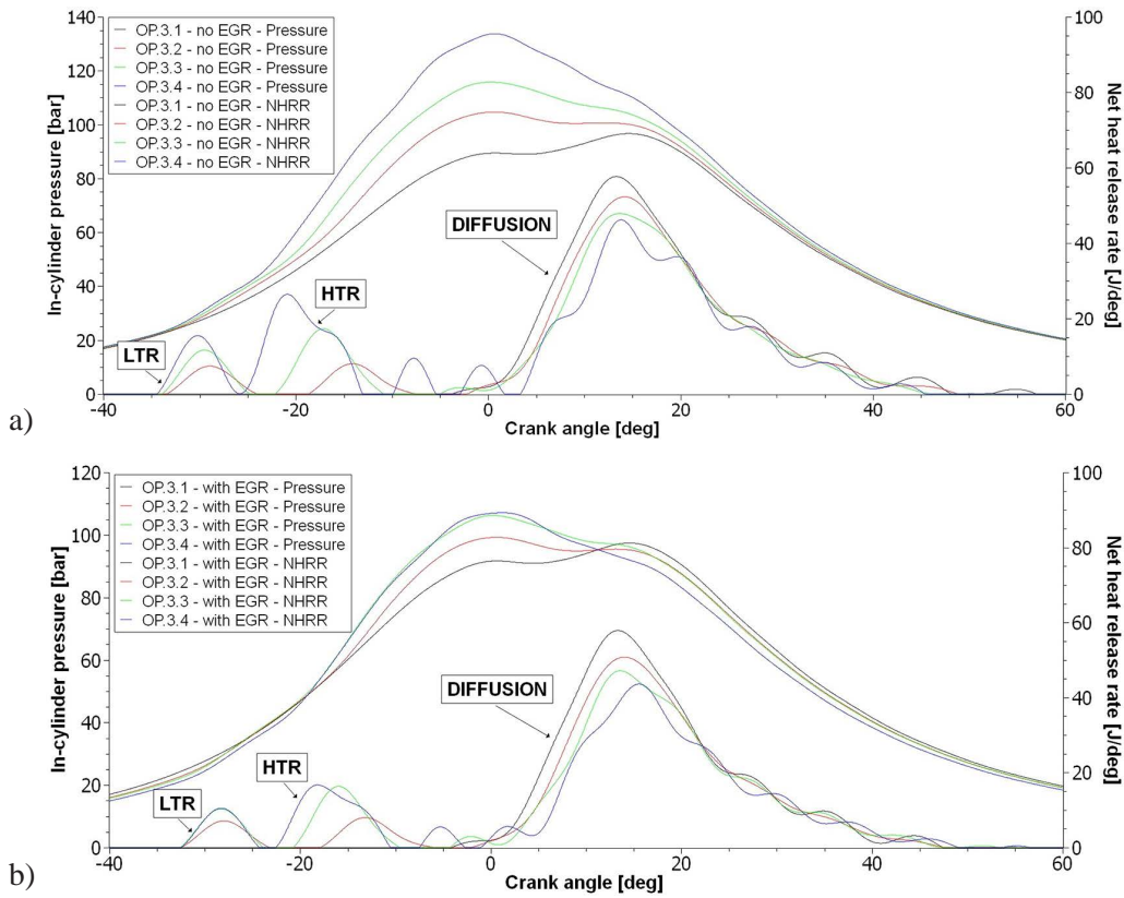
Fig. 7. In-cylinder pressure and net heat release rate variations for OP.3; (a) operation point without EGR, (b) operation point with EGR
