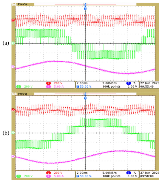
Fig. 19. Waveform of common mode voltage of the three-level, three-phase NPC inverter controlled using the (a) proposed modulation method and (b) CBPWM. CMV: 2) 200 V/div; line-to-line output voltage: 3) 200 V/div; output current: 4) 5 A/div; time scale: 2 ms/div.
