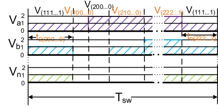
Fig. 8. Switching pattern with replaced zero vectors.
