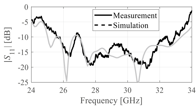
Figure 11. EM-simulated (gray) and measured (black) reflection coefficient.
