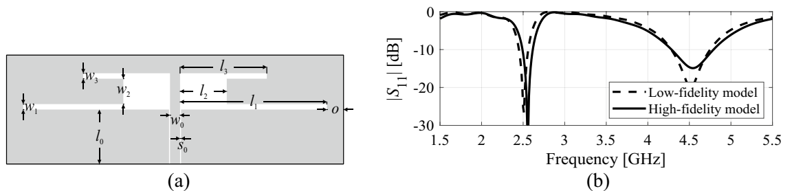
Figure 3. Variable-fidelity models: (a) an exemplary dual-band antenna, (b) its reflection responses evaluated using the low-fidelity EM model (---) and the high-fidelity one (—). In the case shown in the picture, the simulation time of the high-fidelity model is about 90 s, whereas the evaluation of the low-fidelity model only takes about 25 s.
