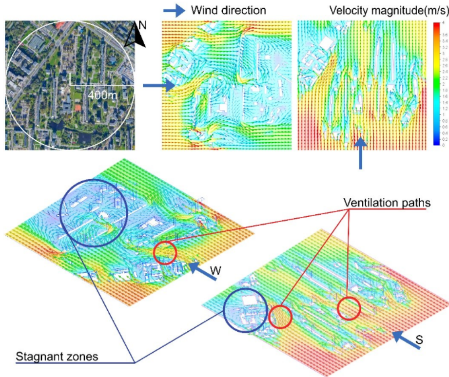
Fig. 10. The results of CFD simulations (velocity magnitude at the height of 2 meters) for selected wind directions (south and west) conducted for the area of interest in the Bielany district. Source: own elaboration, based on: [51].
