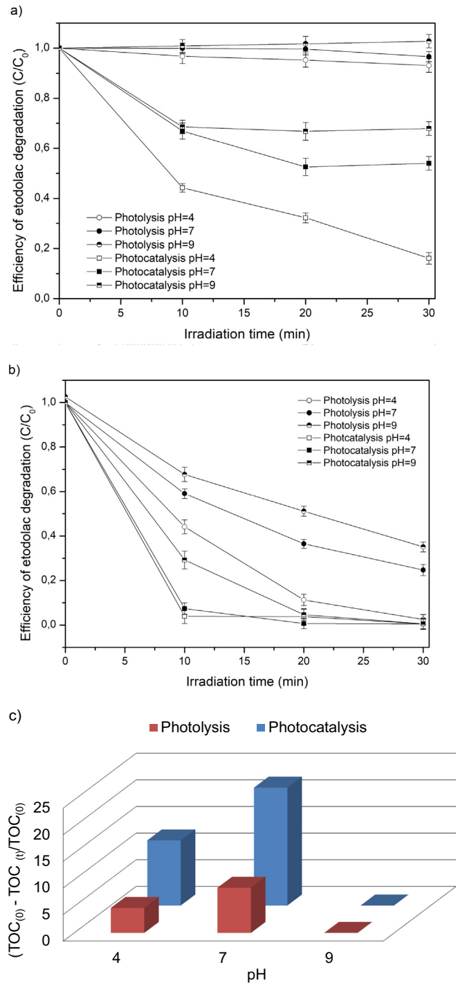
Fig. 9. The effect of initial pH on the etodolac removal under Vis light (a) under UV light (b) and the TOC removal fraction as a function of pH for \text{ZnFe}_2\text{O}_4/\text{SiO}_2/\text{TiO}_2 under UV light irradiation (c).
