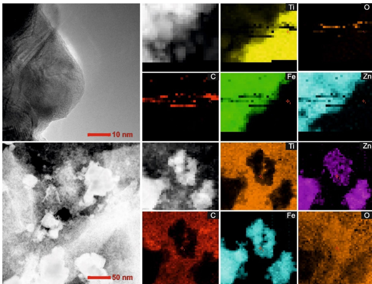
Fig. 4 Morphology (TEM images) and mapping of the 2D/2D \text{TiO}_2 -GO- \text{ZnFe}_2\text{O}_4 photocatalyst
