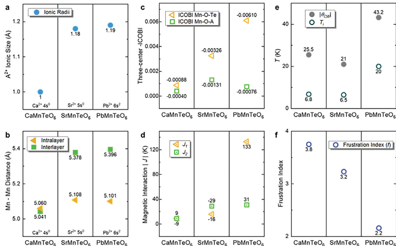
Figure 9. a) Ionic radii of the A sites ( A = \text{Ca} , \text{Sr} , and \text{Pb} ). b) Mn–Mn distances in \text{AMnTeO}_6 . c) Integrated three-center crystal orbital bond index (ICOB) up to E_F for \text{AMnTeO}_6 showing the multicenter intralayer and Mn–O–A interlayer interactions for \text{AMnTeO}_6 showing the comparison of the Mn–O–A interlayer interactions. d) Calculated intralayer J_1 and interlayer J_2 magnetic interactions for \text{AMnTeO}_6 showing the comparison of the Mn–Mn Heisenberg exchange constants. e) Curie–Weiss temperature ( T_i ) and ordering temperature ( T_i ). f) Frustration index ( f ) of \text{AMnTeO}_6 .
