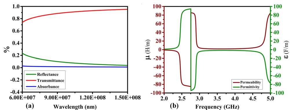
Figure 2. MTM characteristics: (a) transmittance, absorbance, and reflectance, (b) permeability and permittivity.
