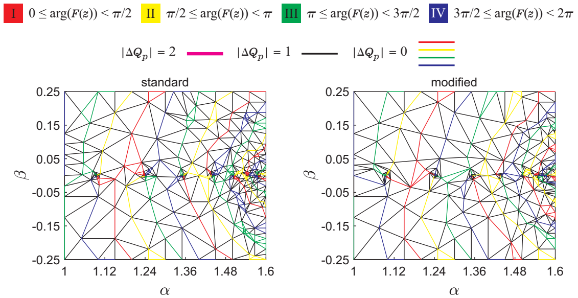
Figure 3.23: The comparison of final meshes for the standard and modified solution of the "skinny" triangle issue.
