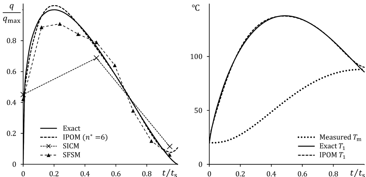
Fig. 9. Inverse problem of contact heat conduction in sliding friction
