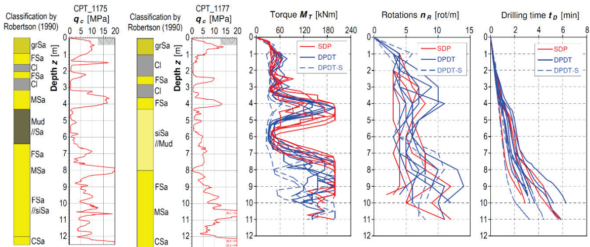
Figure 6. Drilling resistances of pile augers with CPTu diagrams on the field experimental plot No. IIIb.
