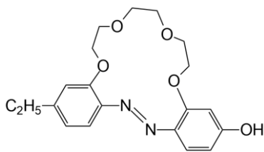
C2-16-p-OH
