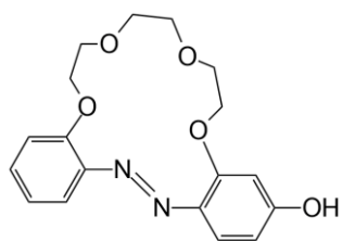
16-p-OH
