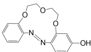
13-p-OH
