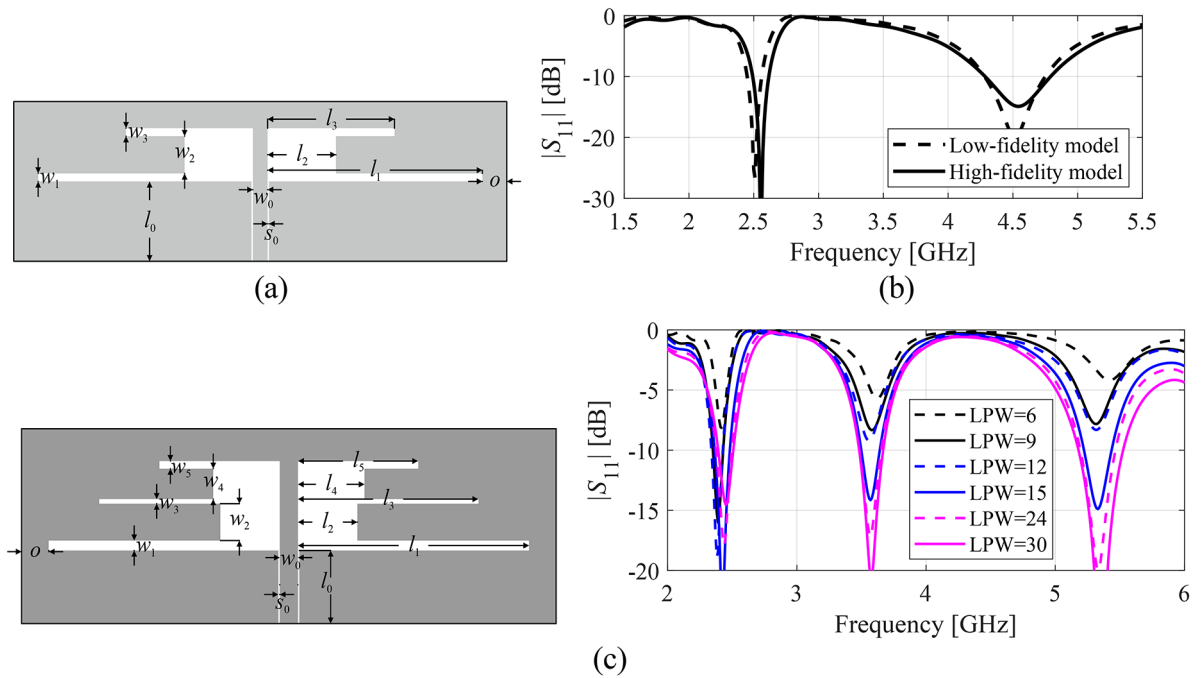
Fig. 1. Multi-resolution EM analysis: (a) a dual-band antenna; (b) |S_{11}| obtained from the low- (---) and high-fidelity EM analysis (—). The high-resolution model simulates in 90 s, whereas the low-fidelity model requires just 25 s of the CPU time; (c) model selection: a triple-band antenna and EM models of various fidelities controlled by lines-per-wavelength (LPW) parameter of CST Microwave Studio. Visual inspection indicates that the models with LPW < 15 are heavily distorted and cannot adequately represent antenna characteristics.
