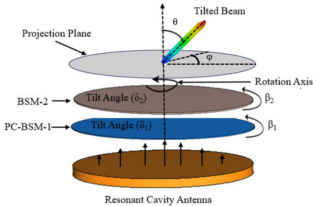
FIGURE 1. The schematic diagram of a beam-steering system with a pair of phase-gradient metasurfaces, rotating PC-BSM-1 and BSM-2, the beam direction is varied in the elevation and azimuth plane.
