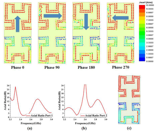
FIGURE 14. (a) axial ratio port 1 (b) axial ratio port 2 (c) vector current distribution.
