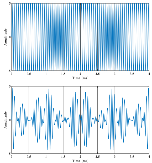
Fig. 8. Transmitted signals a) MFSK ( f_3 ) b) MC-4-4FSK ( f_0, f_4, f_{11}, f_{15} )
