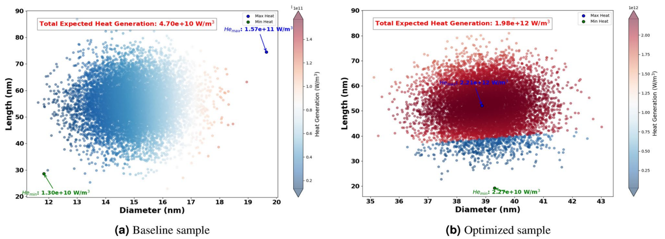
Figure 10. Expected heat generation with baseline (a) vs optimized (b) sample irradiated by \lambda = 532 nm.
