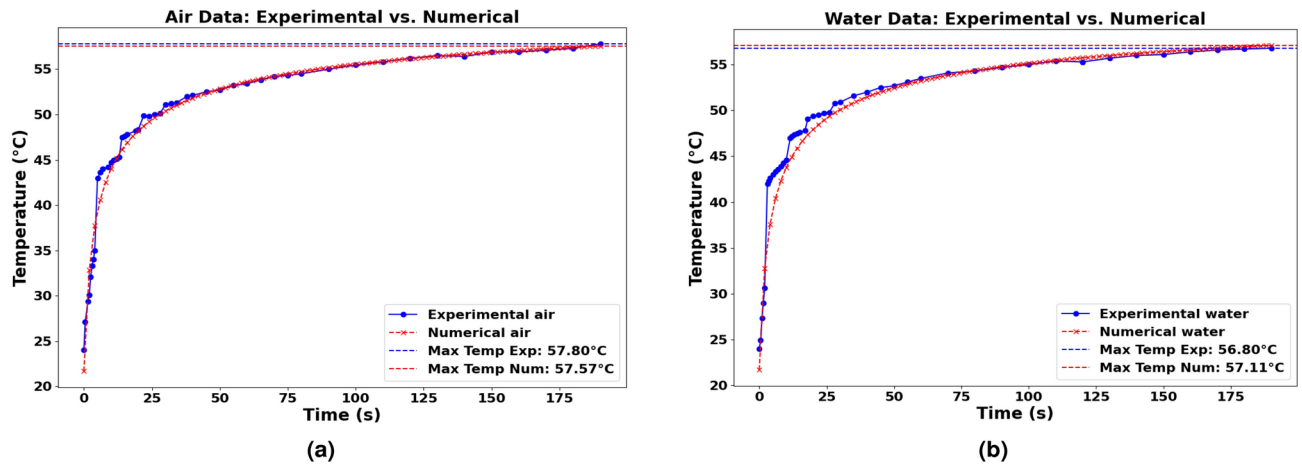
Figure 5. Energy conversion model validation against experimental results for air (a) and water (b) case data comparison.
