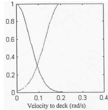
Fig. 11. Input membership functions: Inference system 2.
