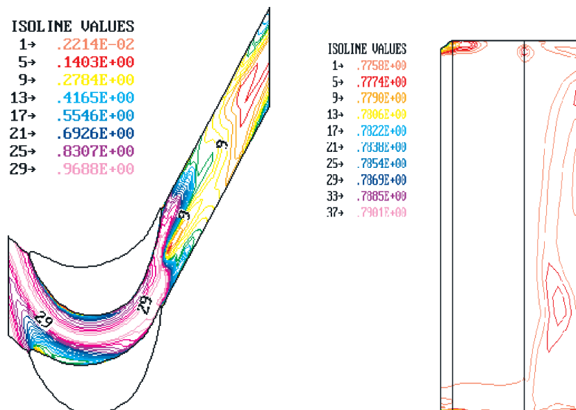
Figure 2. Example of distribution of kinetic energy losses in a blade cascade
