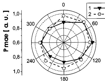
FIG. 4. Polar diagrams of normalized MAE parameter P_{mae} for two directions of magnetization: 1-hoop, 2-axial.
