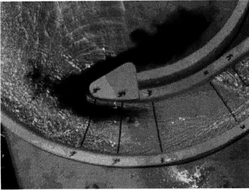
Fig. 9. Water flow between cross-sections v1-v1 and x-x
