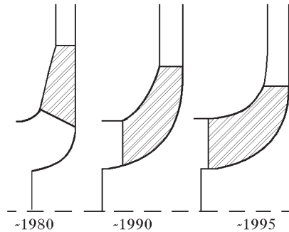
Fig. 1. Evolution of compressor meridional shape
