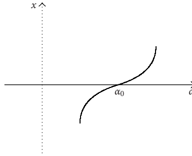
Figure 3.1. Transcritical bifurcation.
