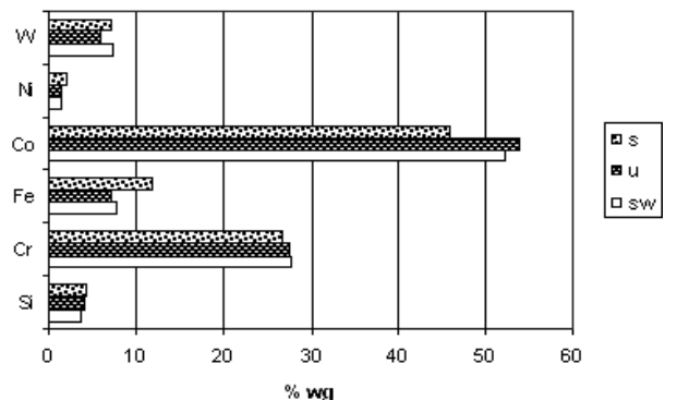
Fig. 2. Chemical analysis (EDS) of the microregions in the middle part of the layer made by laser cladding
