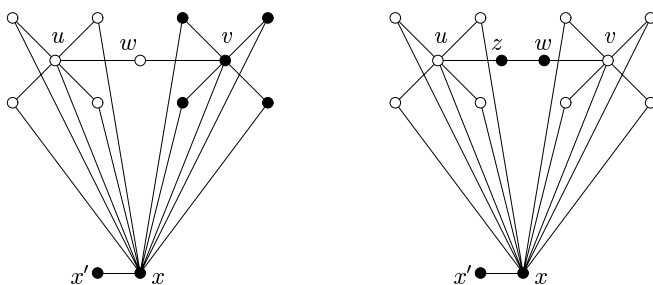
Figure 2: Graphs H and H \oplus z_{uv} for k=5
