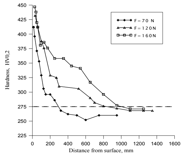
Fig. 4. Hardness distribution at surface layers of duplex stainless steel samples after burnishing
