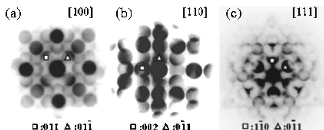
FIG. 2. Convergent beam electron diffraction patterns for Mg_{10}Ir_{19}B_{16} along (a) [100] , (b) [110] , (c) [111] show clearly 4 mm, m , 3 m symmetry, respectively. This indicates that the space group of the material is I-43m .
