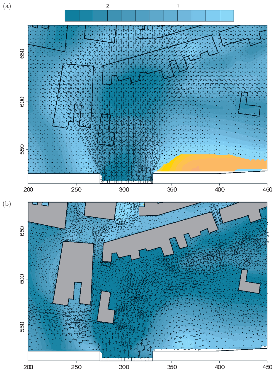
Figure 10. Test case 2: detail of computed contours of water depth and flow directions after t = 180\text{s} of simulation for test case 2a (a) and 2b (b) (dimensions and depth in metres)
