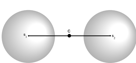
Figure 4. The initial configuration of the macroscopic model of two entangled spin 1/2 in the singlet state.
