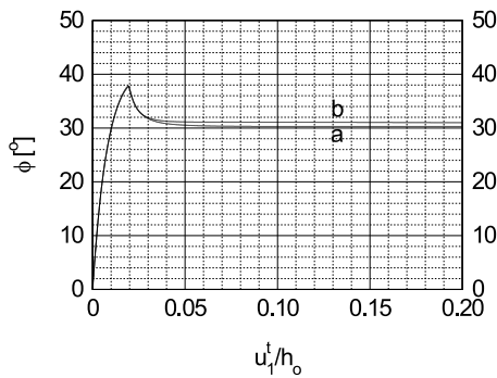
Fig. 12. Evolution of mobilized internal friction angle \phi versus u_1^t/h_o during shearing with dense sand ( \bar{e}_o = 0.60 , correlated random field of e_o , approach 'B'): a) s_d = 0.05 , \lambda_{x1} = \lambda_{x2} = 1 , b) s_d = 0.05 , \lambda_{x1} = \lambda_{x2} = 3
