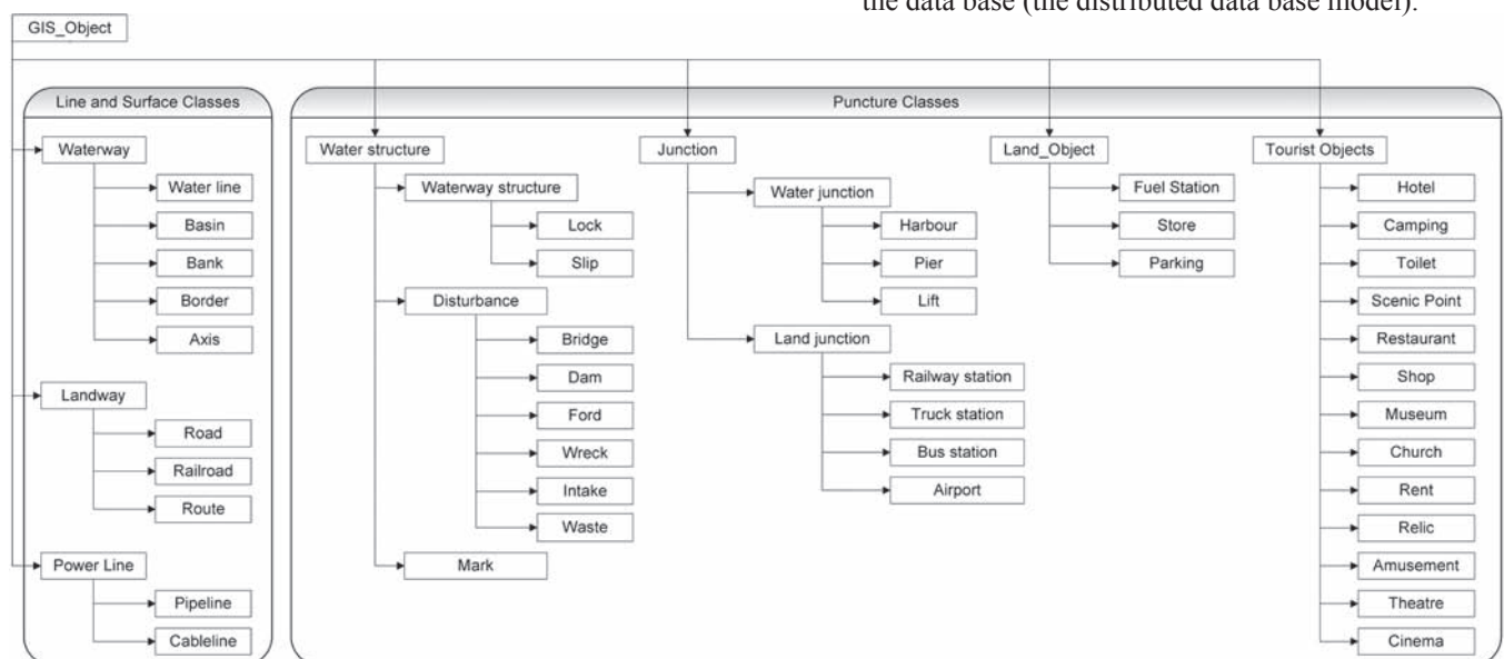
Fig. 5. Hierarchy of classes of the assumed GIS model .
